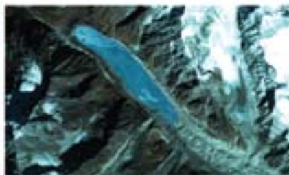
19 January 2007, AVNIR-2
