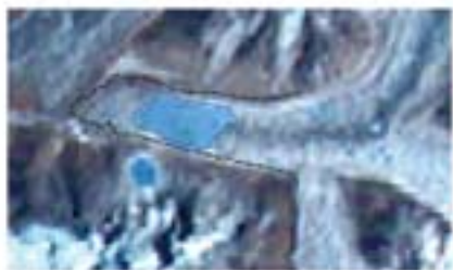
9 April 1984, Landsat 4
