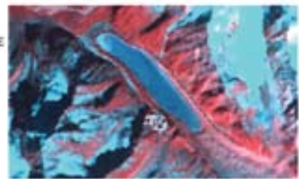
15 January 1999, LISS-3
